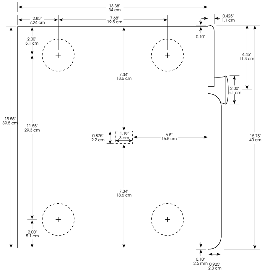
Dimensions, N°38S, top view
