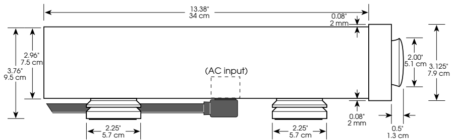
Dimensions, N°38S, side view
