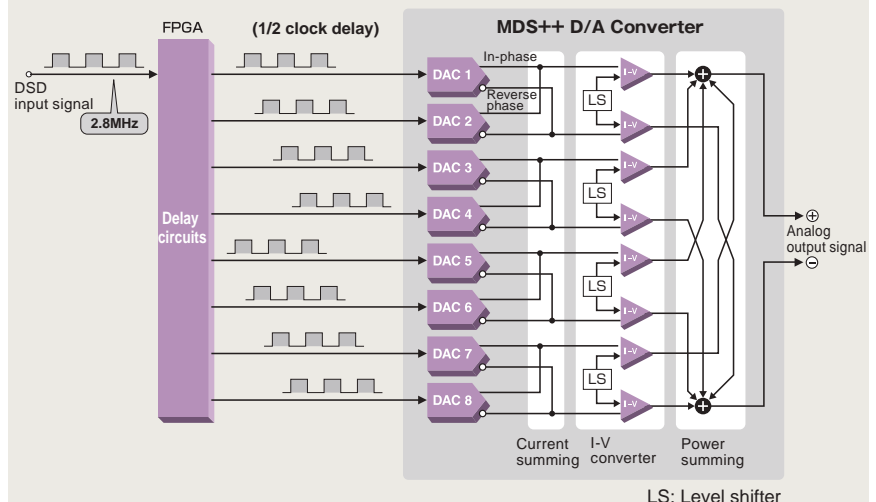
MDSD principle block diagram
