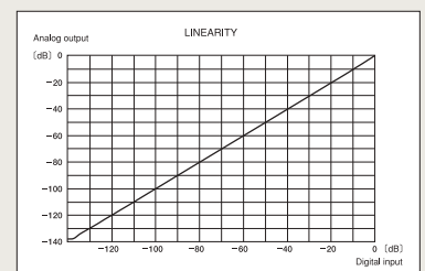
Linearity (digital input vs. analog output)
